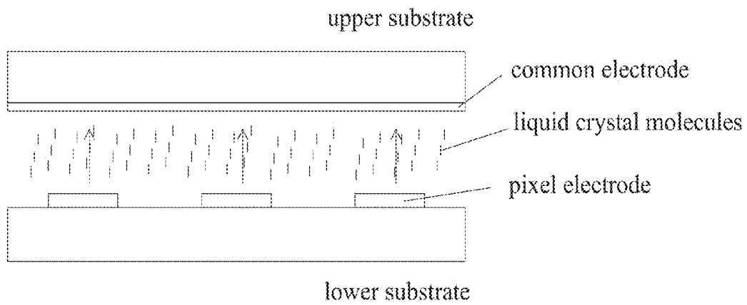
Fig. 1C (Prior Art)
