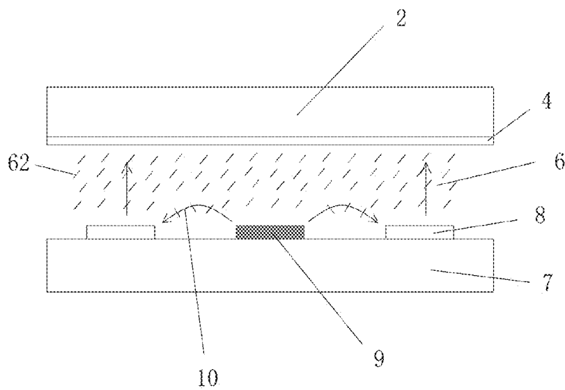
Fig. 1C (Prior Art)
