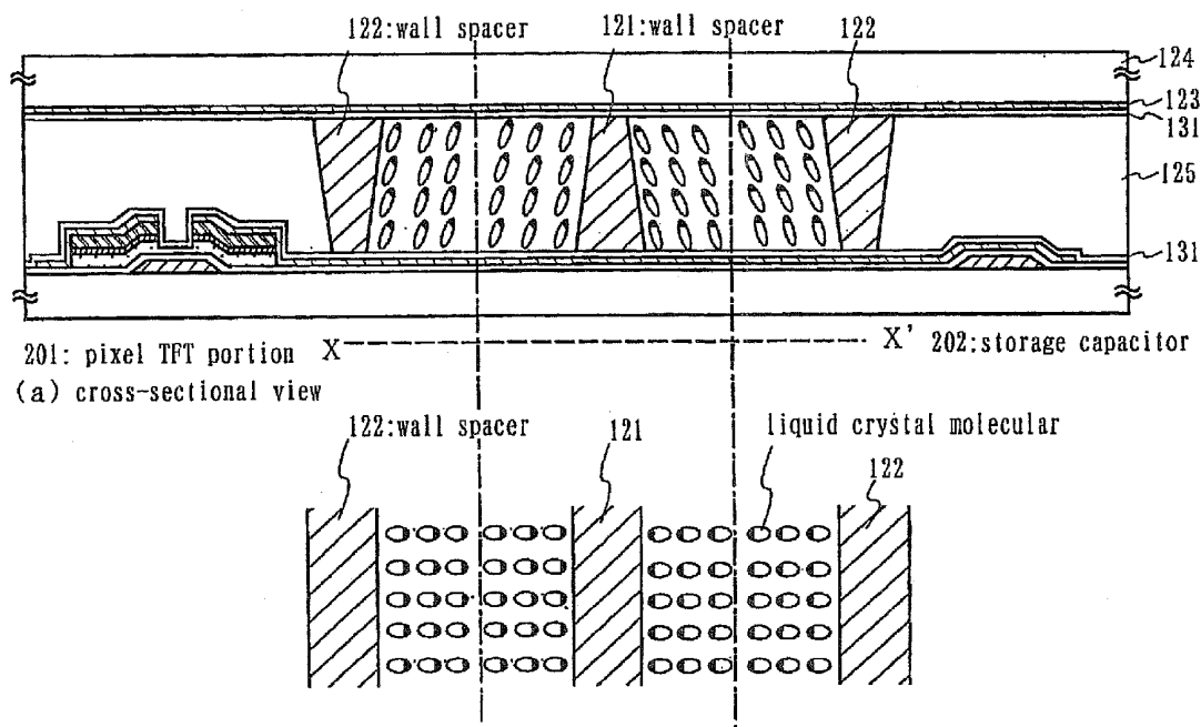
(b) liquid crystal molecule orientation state
