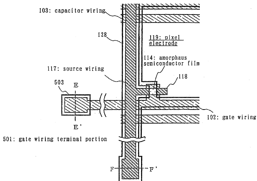
(A) top view 502: source wiring terminal portion
