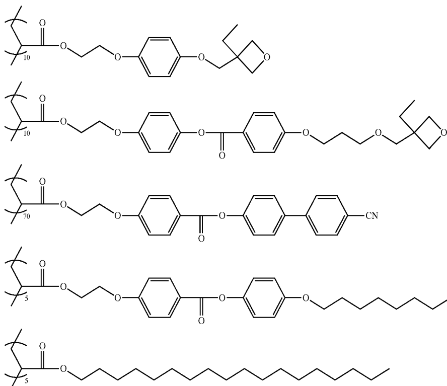
[Chem. 2]
