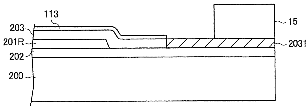
FIG. 16 PRIOR ART
