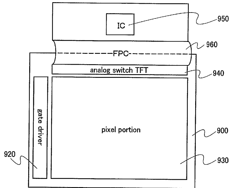
FIG. 17A IC connected by FPC
