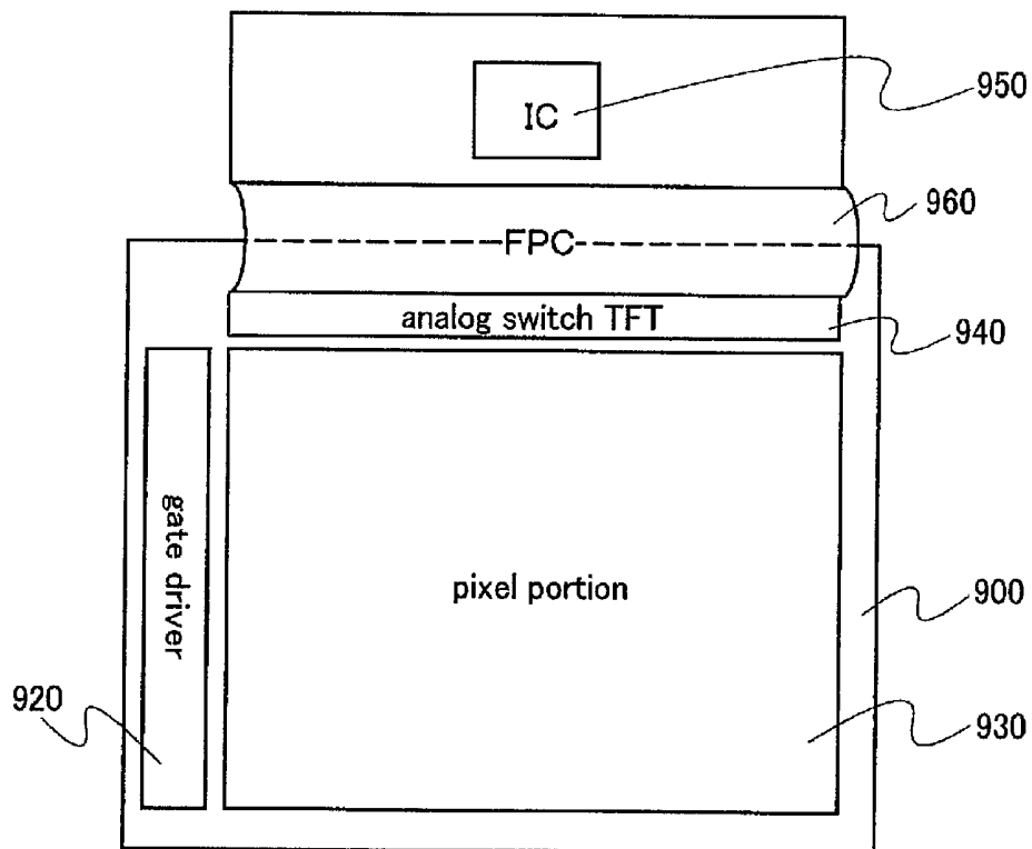
FIG. 17A IC connected by FPC
