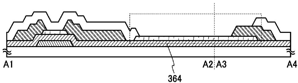
FIG. 12D
