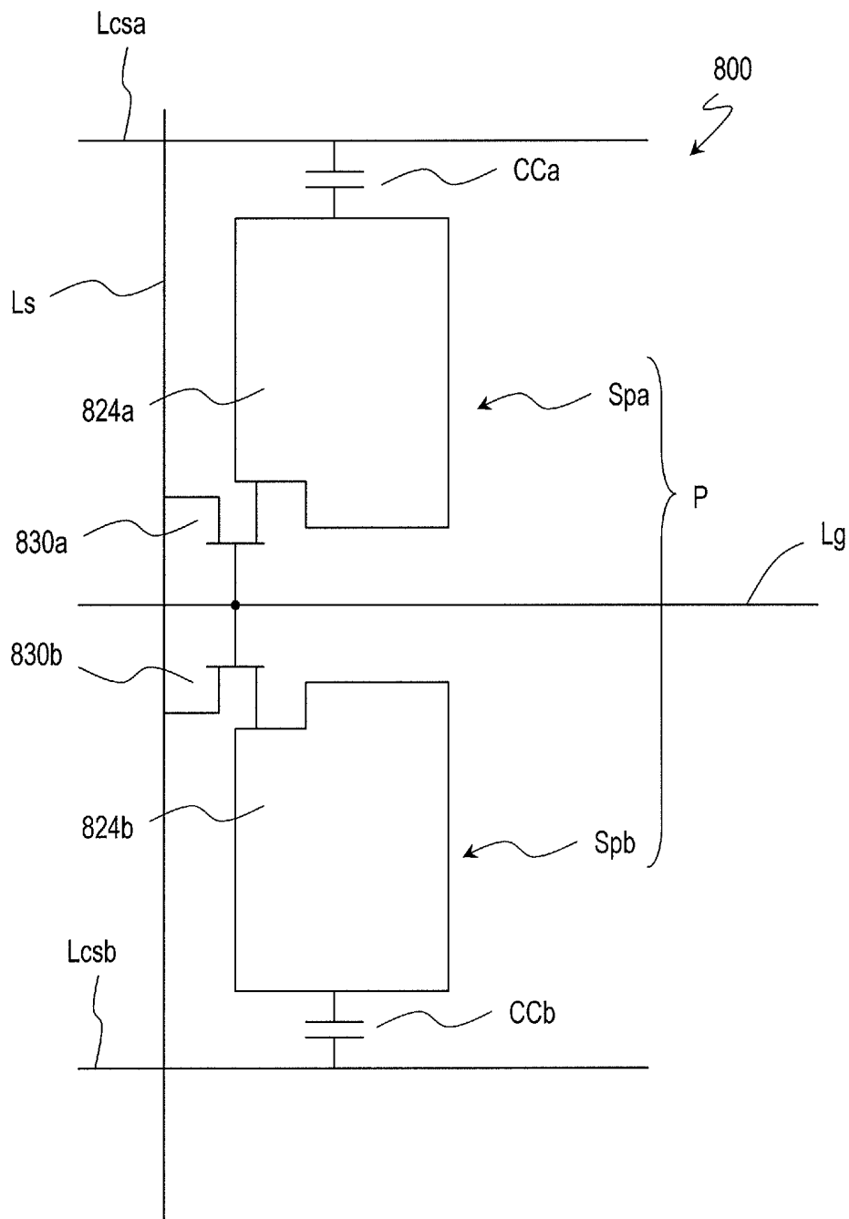
FIG. 9 PRIOR ART
