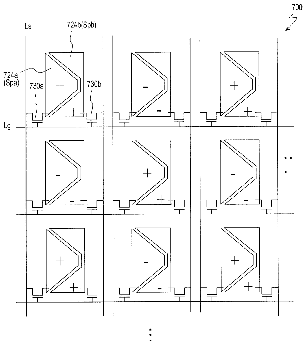
FIG. 8 PRIOR ART
