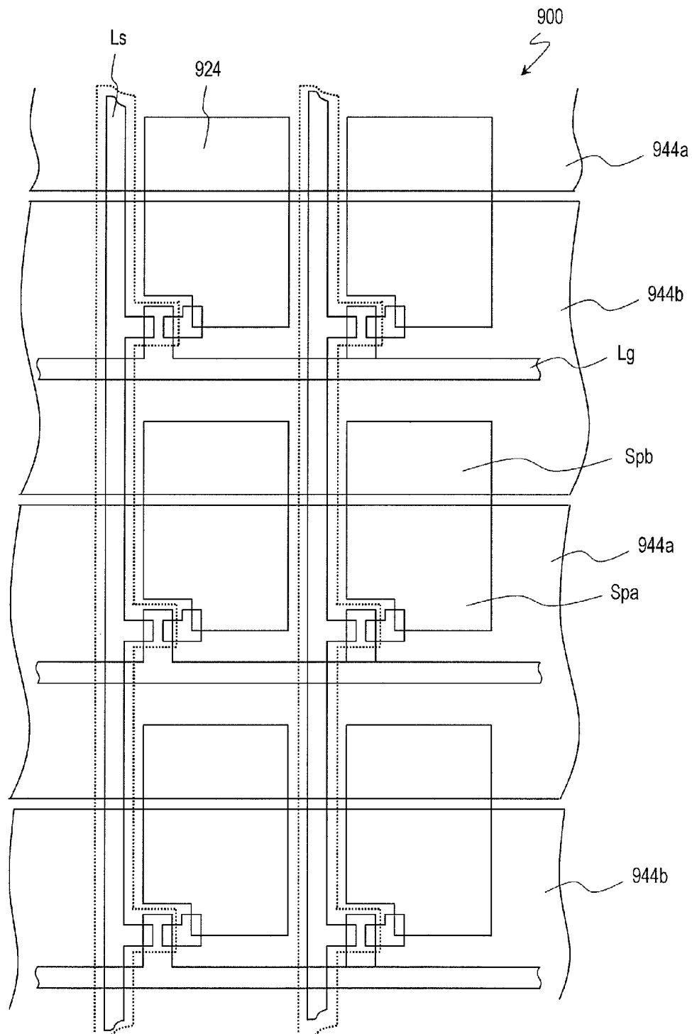
FIG. 10 PRIOR ART
