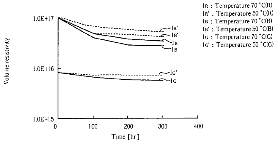
Fig. 9 Prior art
