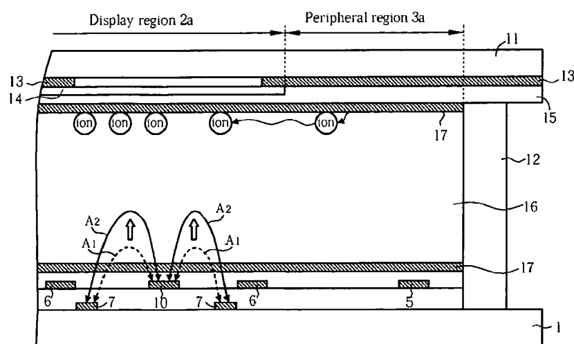
Fig. 4 Prior art
