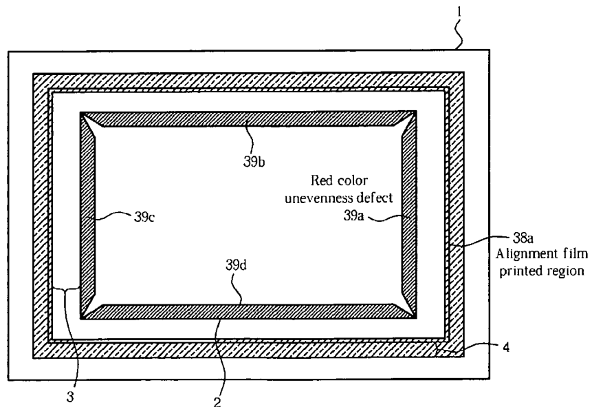
Fig. 12 Prior art
