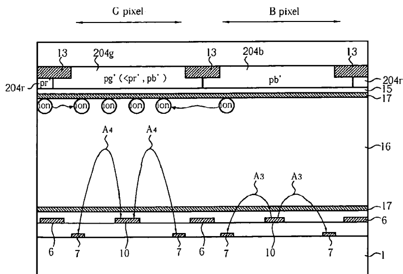
Fig. 10 Prior art
