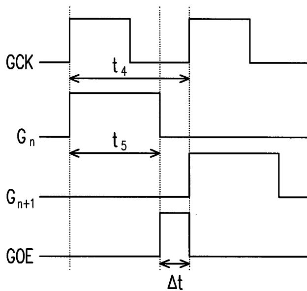
FIG. 4 (PRIOR ART)
