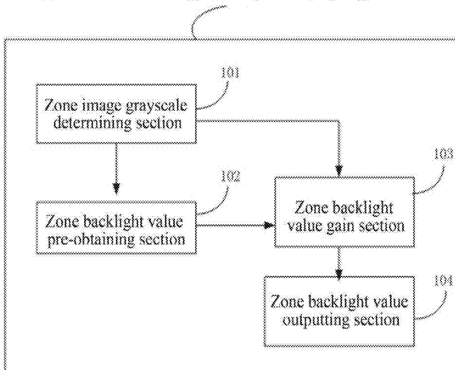
Apparatus for controlling liquid crystal display brightness10
