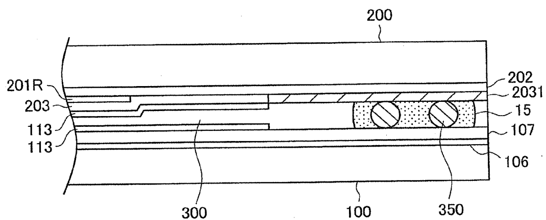
FIG. 17 PRIOR ART
