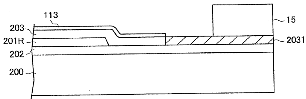
FIG. 16 PRIOR ART
