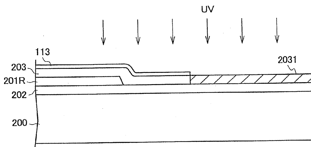
FIG. 15 PRIOR ART
