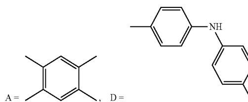
[Chemical formula 4]
