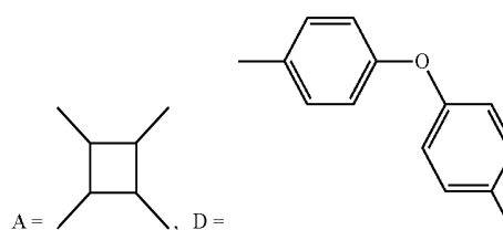
[Chemical formula 3]
