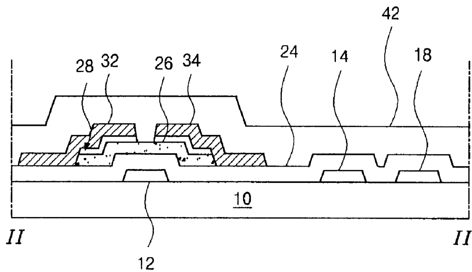
FIG. 2C (Related Art)
