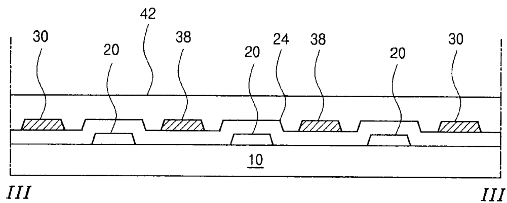
FIG. 3C (Related Art)
