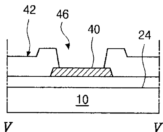
FIG. 5C (Related Art)
