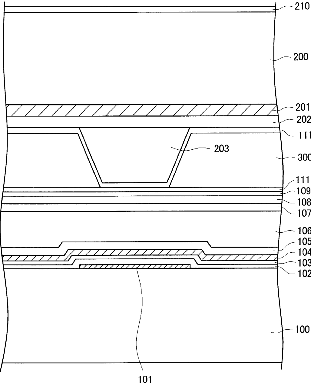
FIG. 7 (Prior Art)
