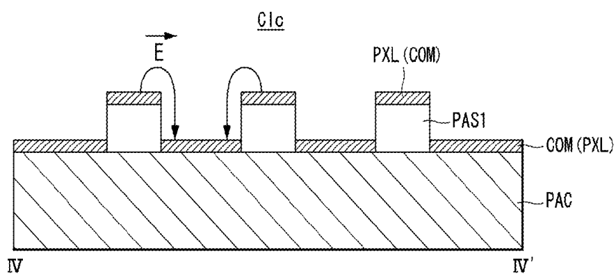
FIG. 17 RELATED ART
