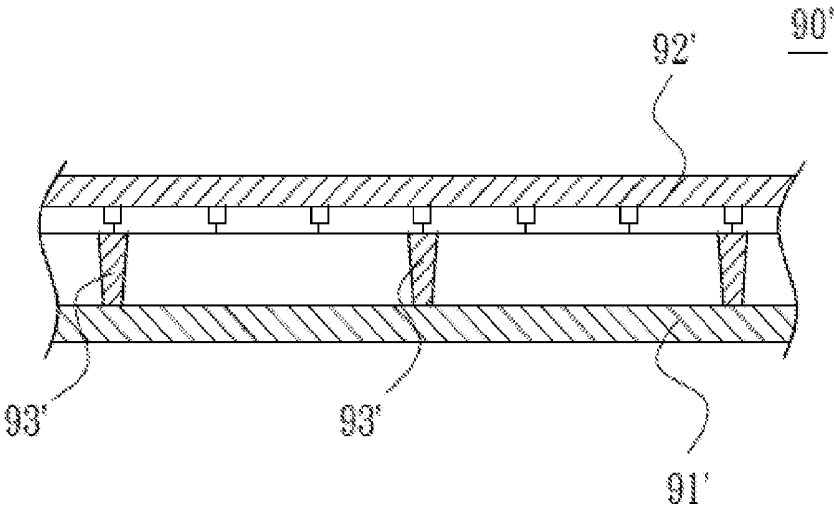
FIG.2 PRIOR ART
