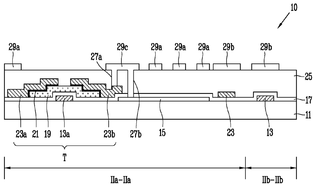
FIG. 2 RELATED ART
