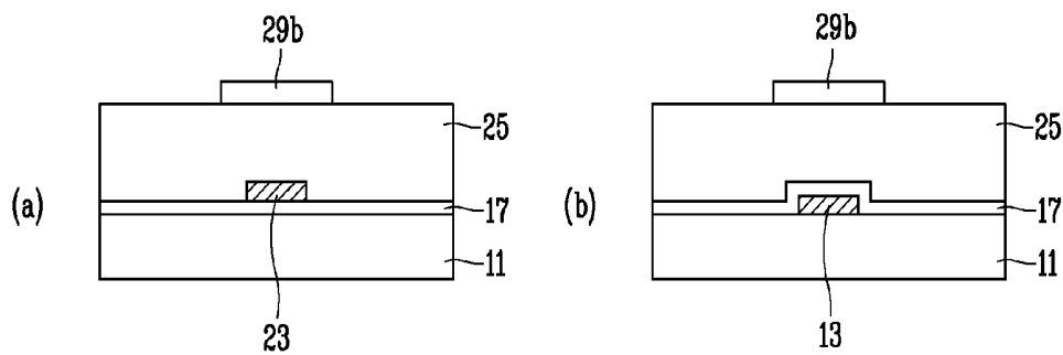
FIG. 3 RELATED ART
