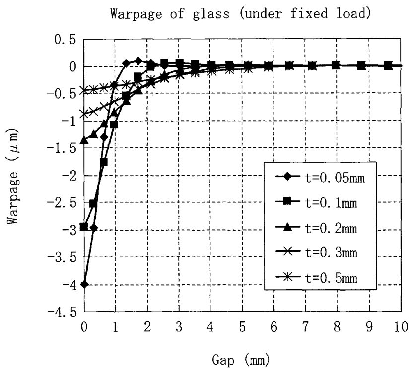
FIG. 15 PRIOR ART
