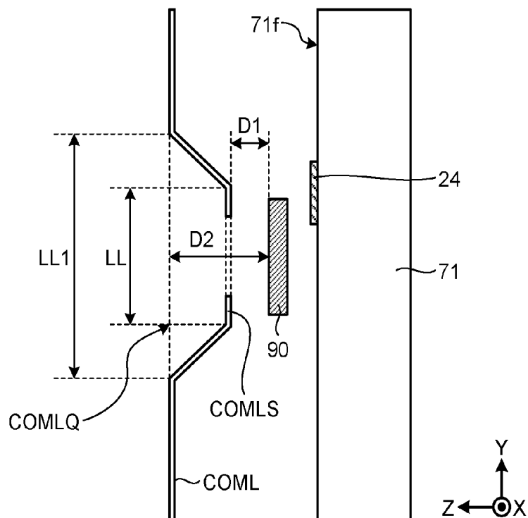
FIG.25 RELATED ART
