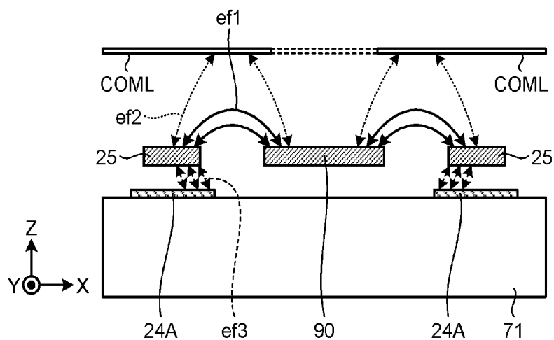
FIG.7 RELATED ART
