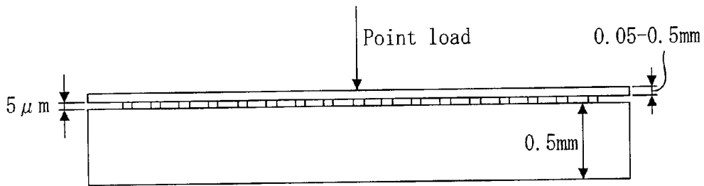
FIG. 14 PRIOR ART
