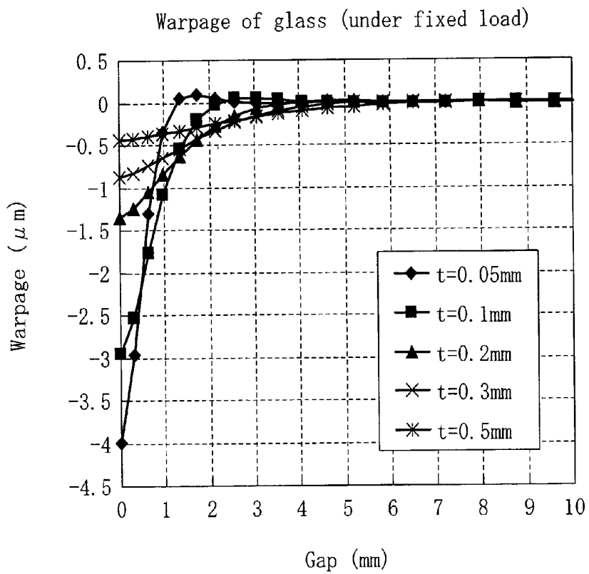
FIG. 15 PRIOR ART
