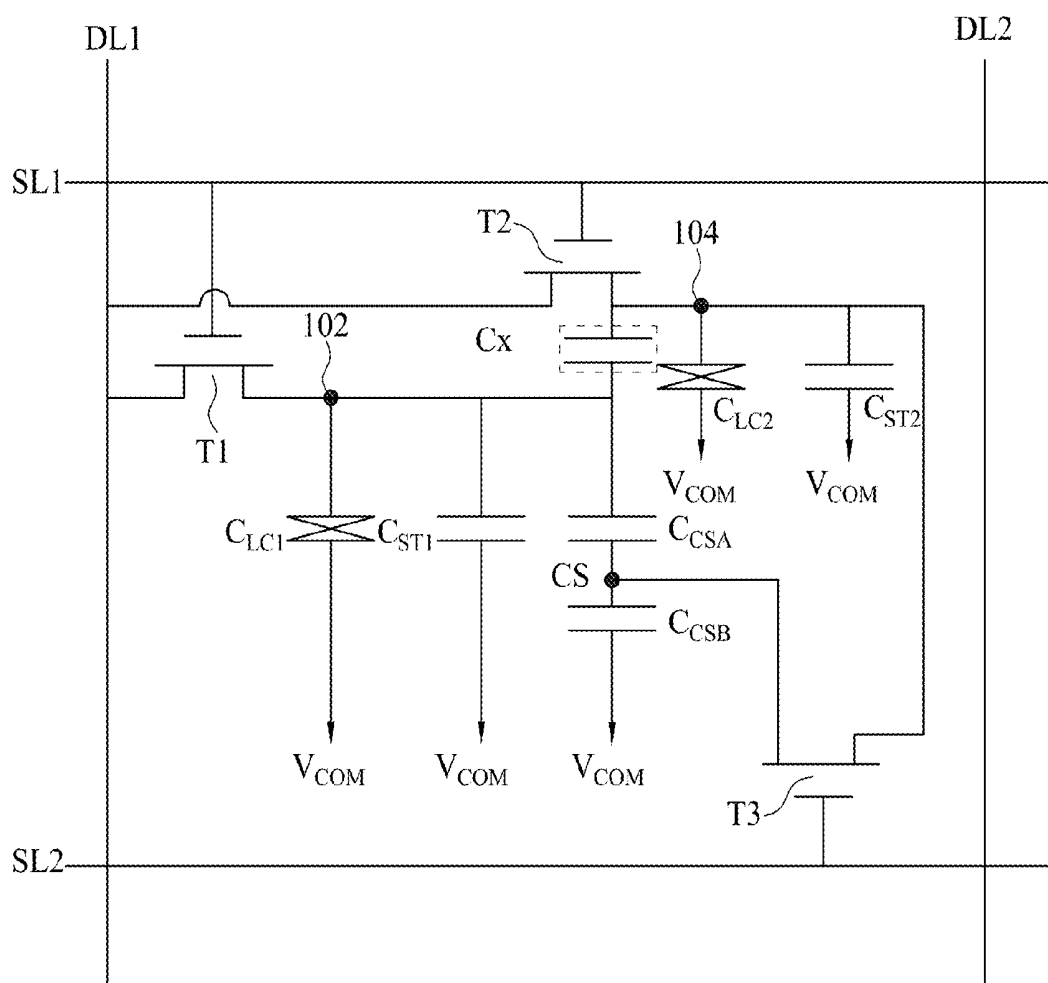
FIG. 2 (PRIOR ART)
