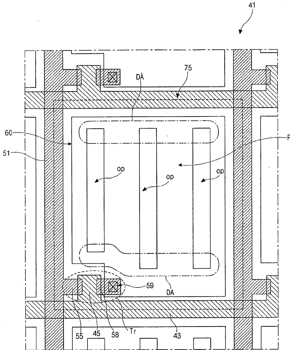
FIG. 3 RELATED ART
