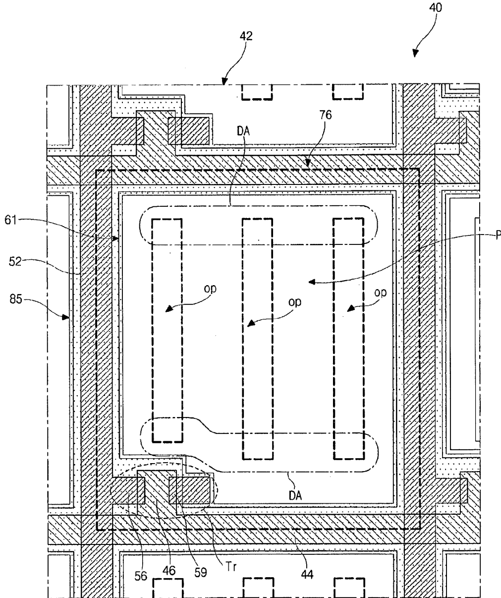
FIG. 5 RELATED ART
