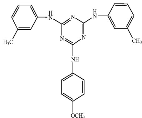
Compound (I-2)
