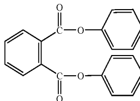
Compound E-15:
