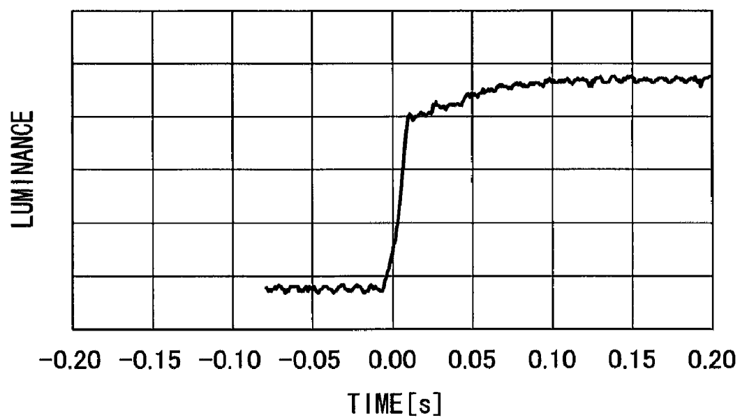
RESPONSE WAVEFORM 0→64
