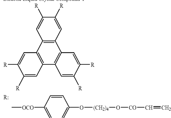
Discotic Liquid Crystal Compound-1
