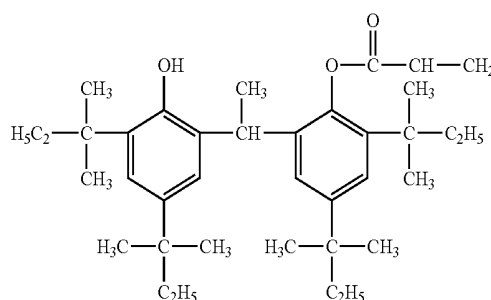
Compound S
