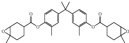
Compound e
