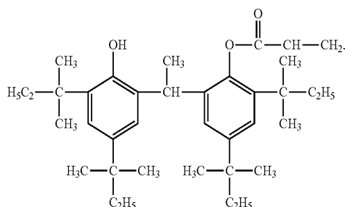
Compound S
