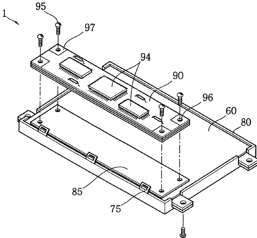
FIG. 2 (PRIOR ART)
