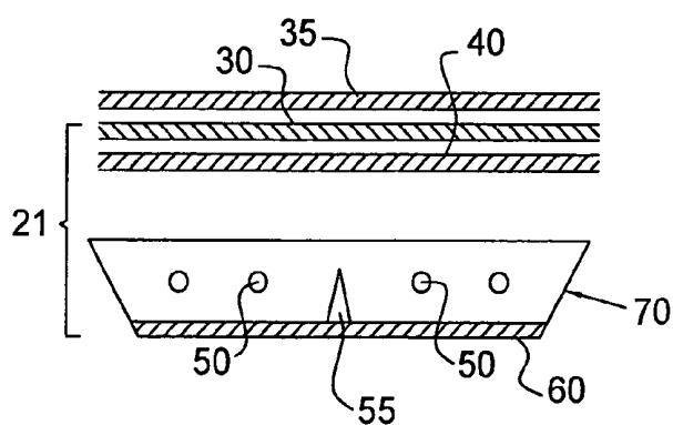
FIG. 2 (PRIOR ART)
