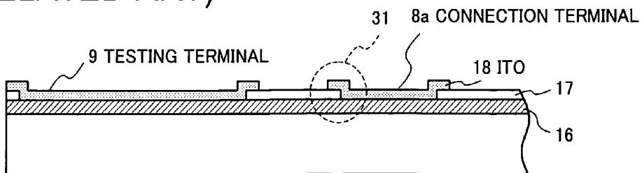
FIG.10C (RELATED ART)
