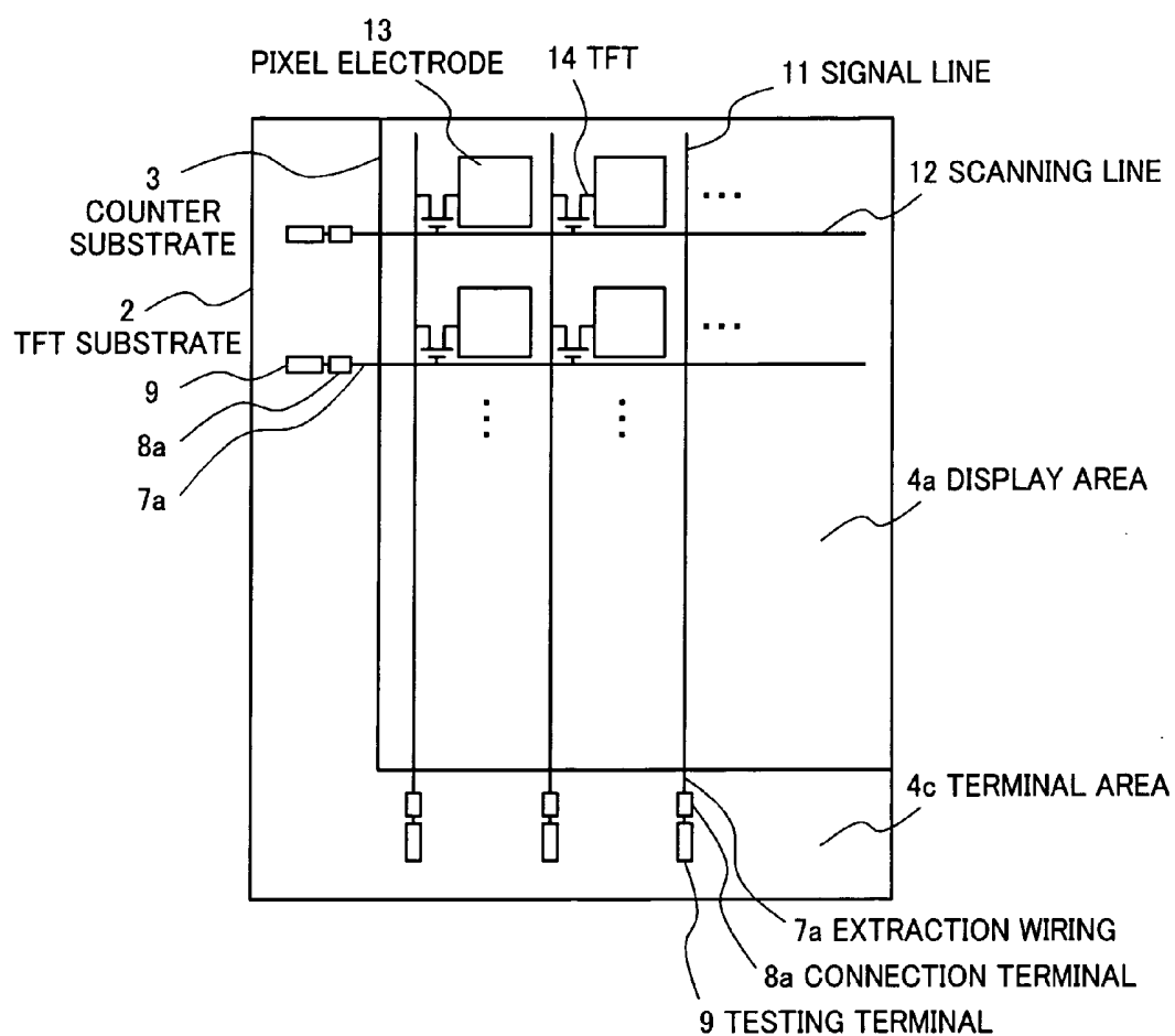
FIG.8 (RELATED ART)
