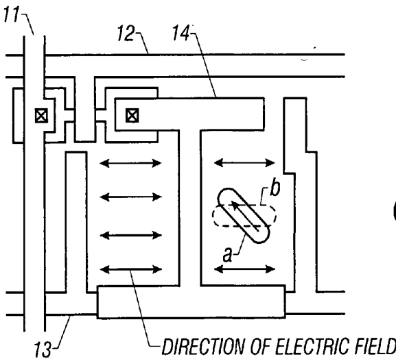
FIG. 6 (Prior Art)
