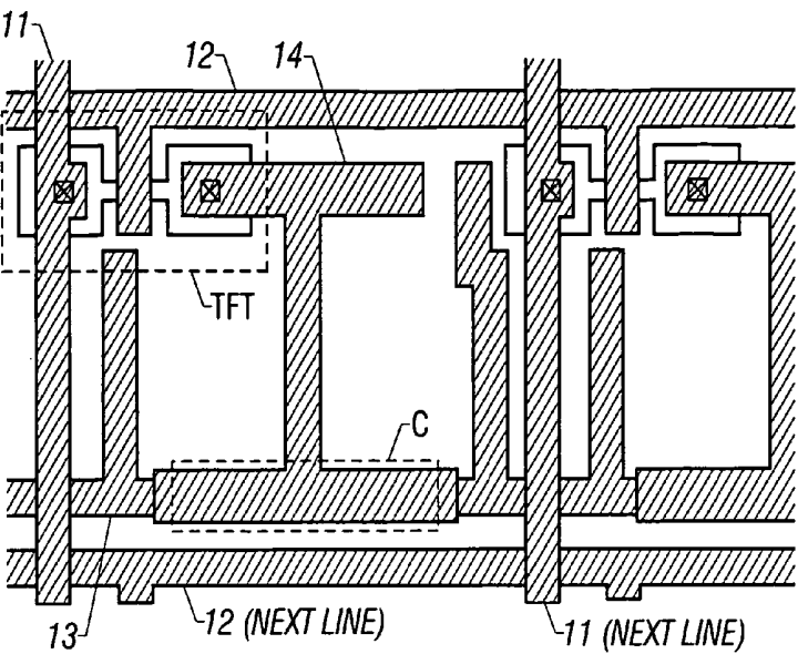
FIG. 5 (Prior Art)
