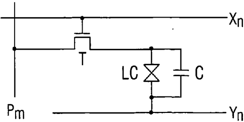
FIG. 7 (Prior Art)
