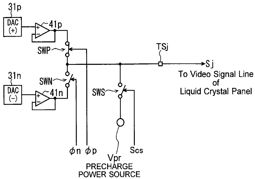
Fig. 15 PRIOR ART
