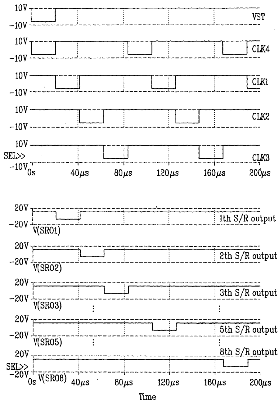
FIG.3 Related Art
