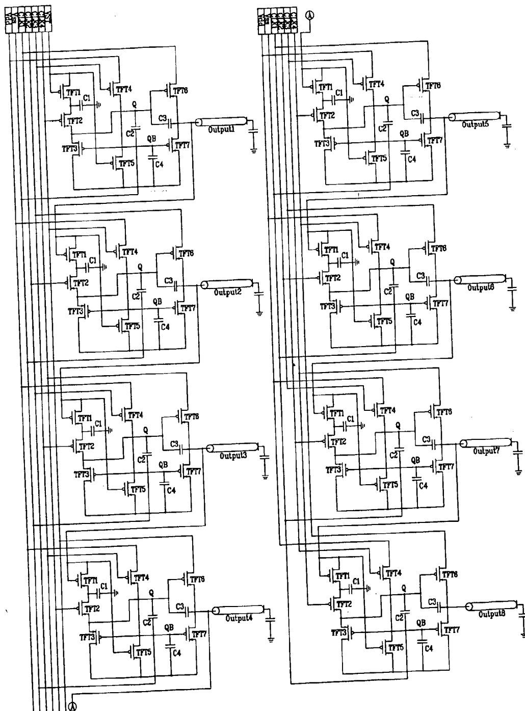
FIG.2 Related Art
