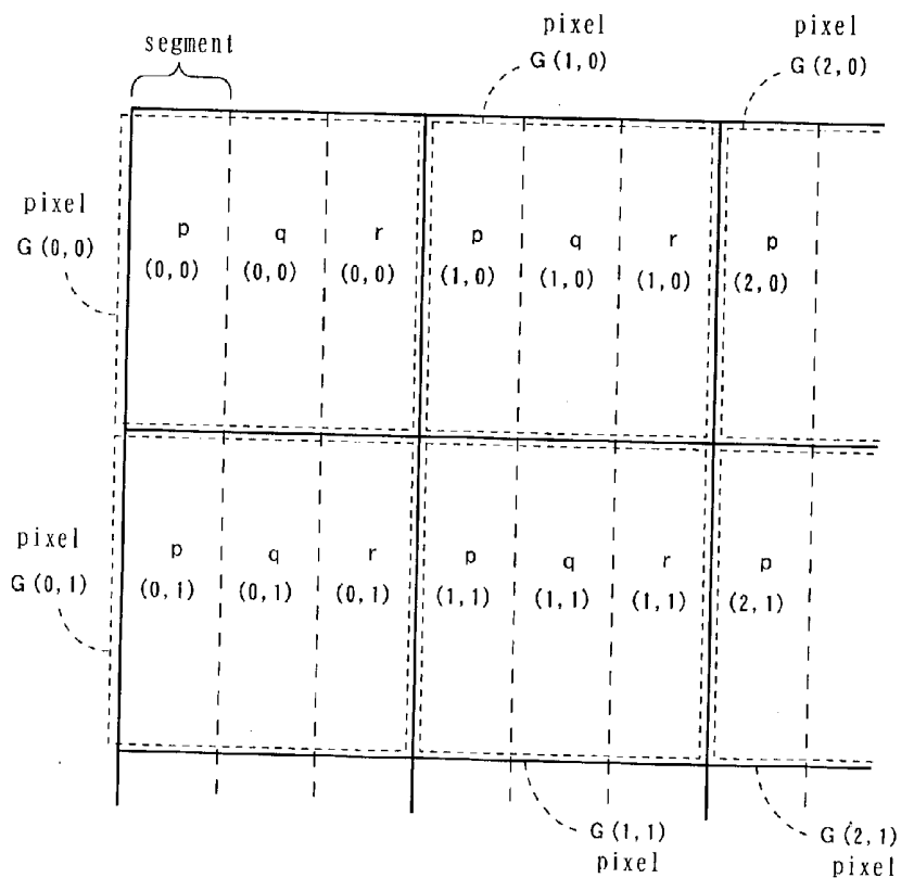
Fig. 6 256 gray scale three-segment monochrom liquid crystal display panel 2 4
