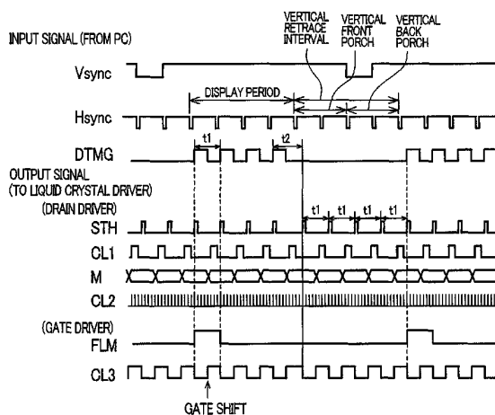
SEQUENCE OF THE LIQUID CRYSTAL DRIVER (EXAMPLE)
