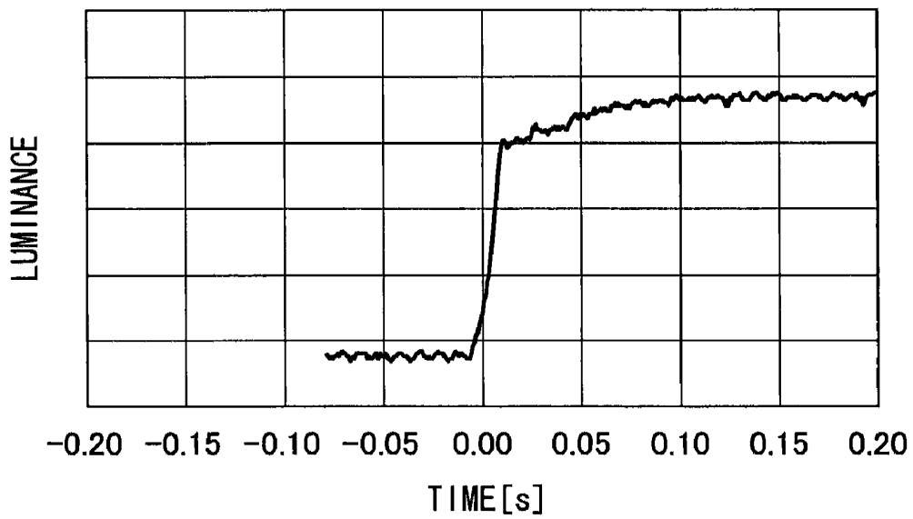
RESPONSE WAVEFORM 0→64
