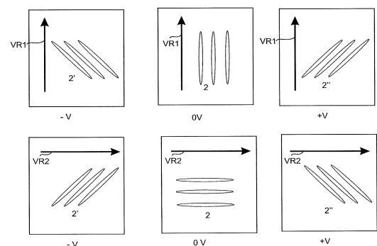
PSS with switchable surface orientation (VR1 -> VR2) and all up 180° settable turning angle of the LC molecules 2
