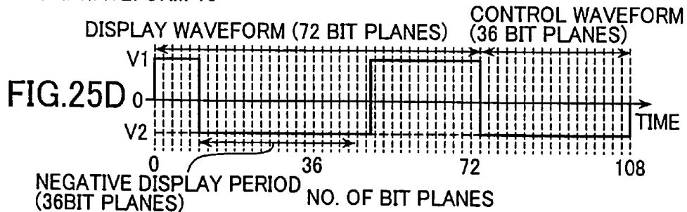
DRIVE WAVEFORM 16
