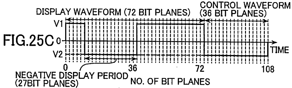
DRIVE WAVEFORM 15
