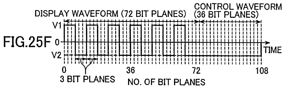
DRIVE WAVEFORM 18
