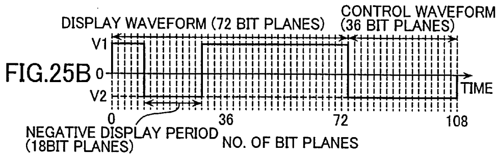
DRIVE WAVEFORM 14
