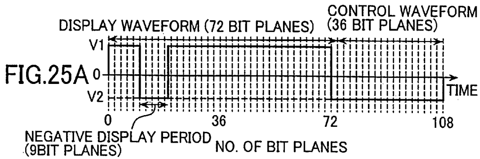
DRIVE WAVEFORM 13
