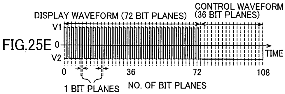
DRIVE WAVEFORM 17
