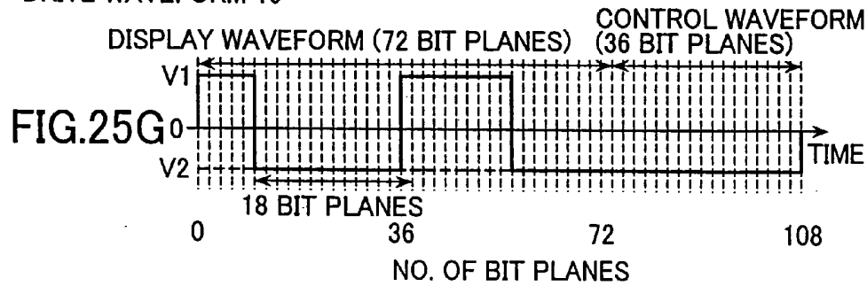
DRIVE WAVEFORM 19
