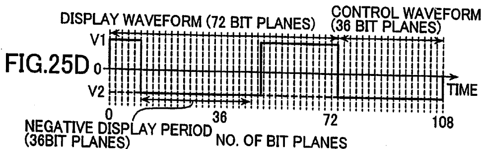
DRIVE WAVEFORM 16
