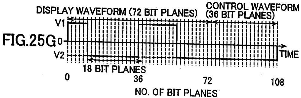
DRIVE WAVEFORM 19
