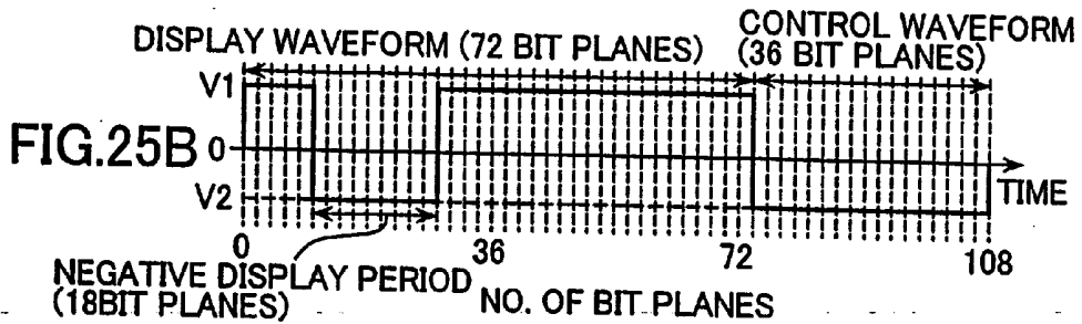
DRIVE WAVEFORM 14
