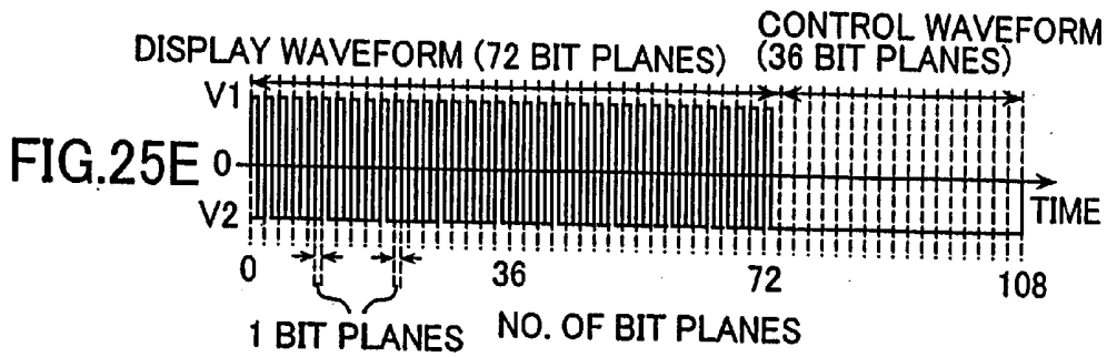
DRIVE WAVEFORM 17
