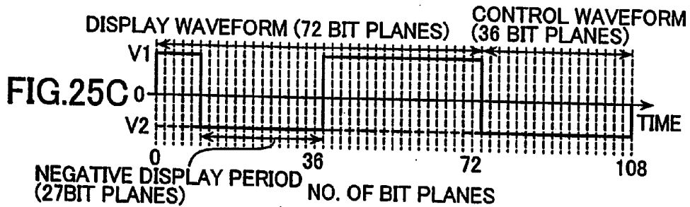
DRIVE WAVEFORM 15
