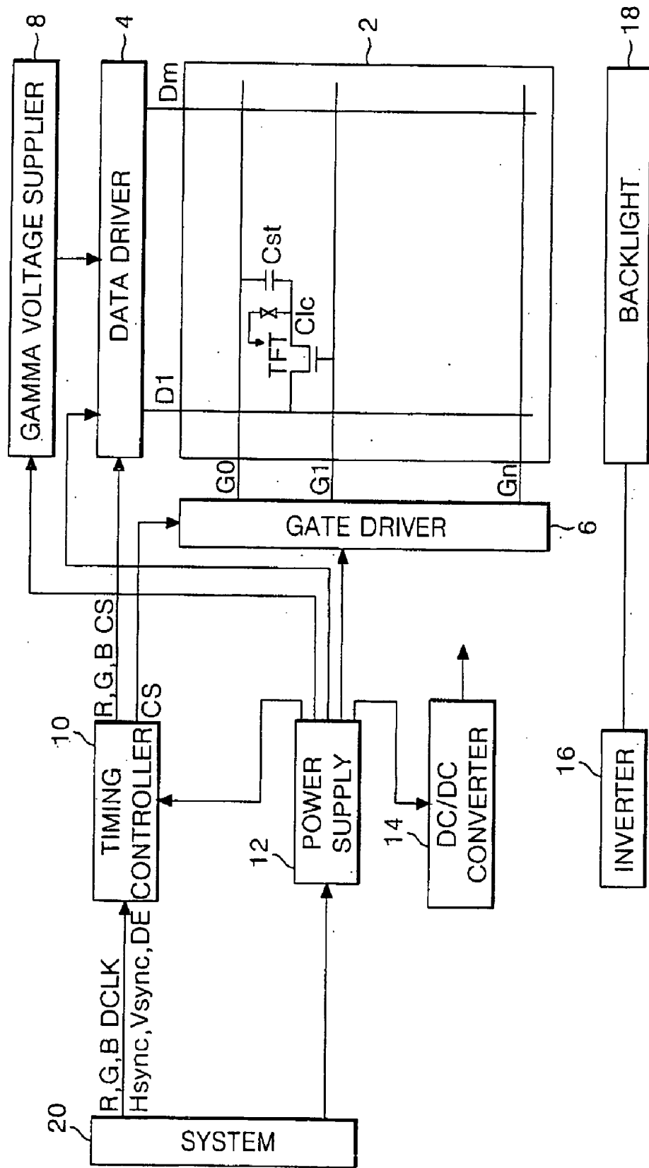
FIG. 1 RELATED ART
