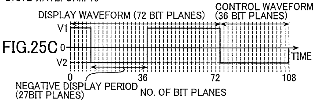
DRIVE WAVEFORM 15
