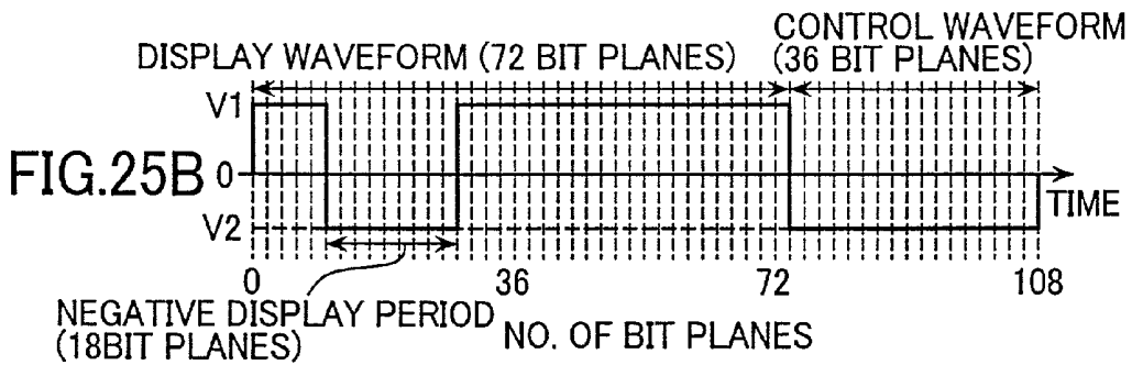
DRIVE WAVEFORM 14
