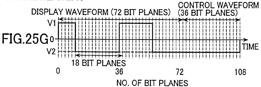
DRIVE WAVEFORM 19
