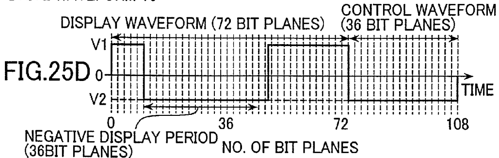
DRIVE WAVEFORM 16
