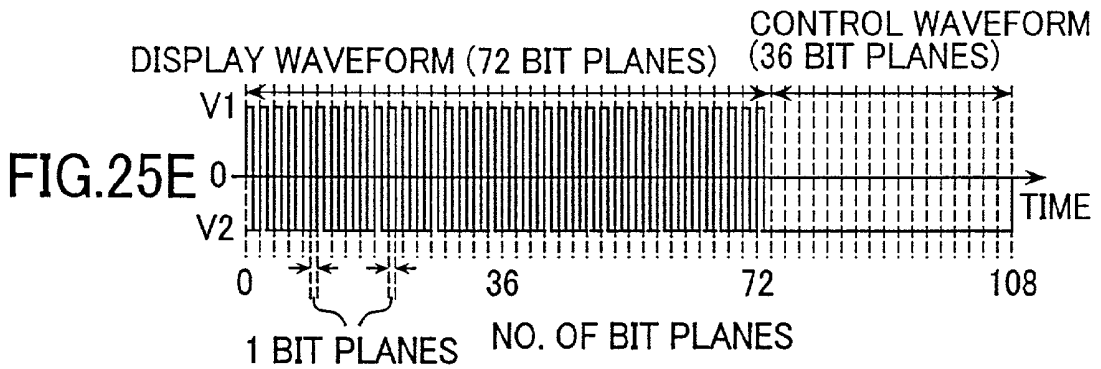
DRIVE WAVEFORM 17
