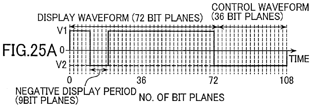
DRIVE WAVEFORM 13
