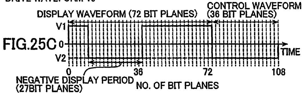
DRIVE WAVEFORM 15
