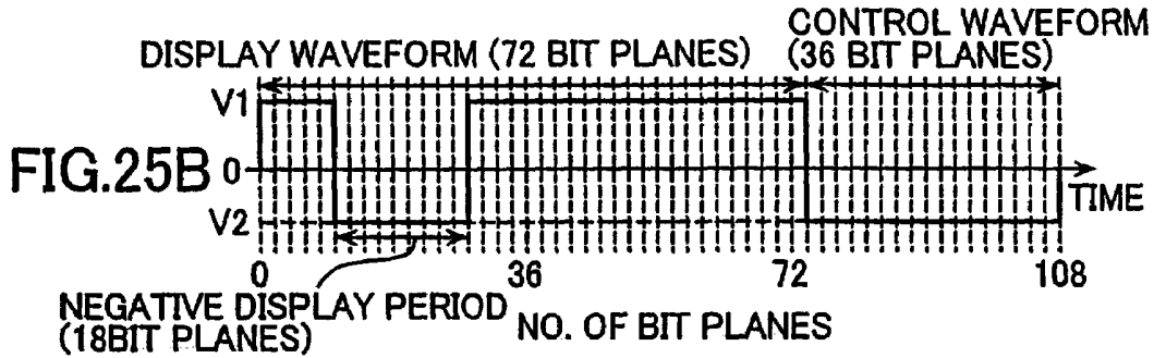
DRIVE WAVEFORM 14
