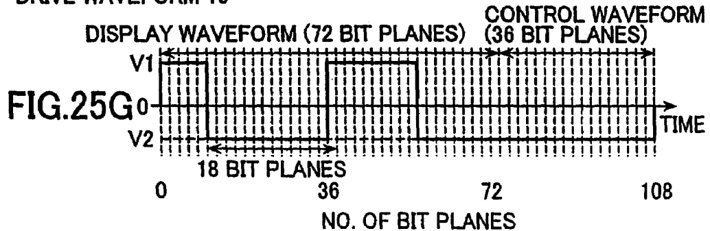
DRIVE WAVEFORM 19
