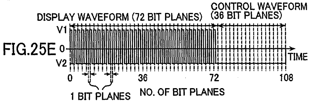
DRIVE WAVEFORM 17
