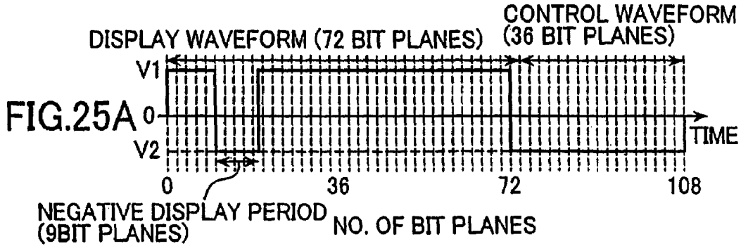
DRIVE WAVEFORM 13
