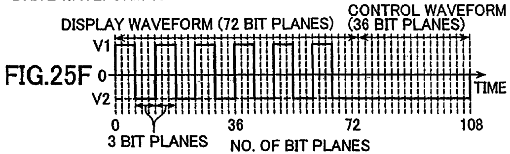
DRIVE WAVEFORM 18
