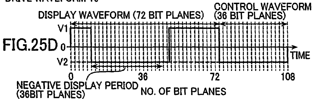
DRIVE WAVEFORM 16
