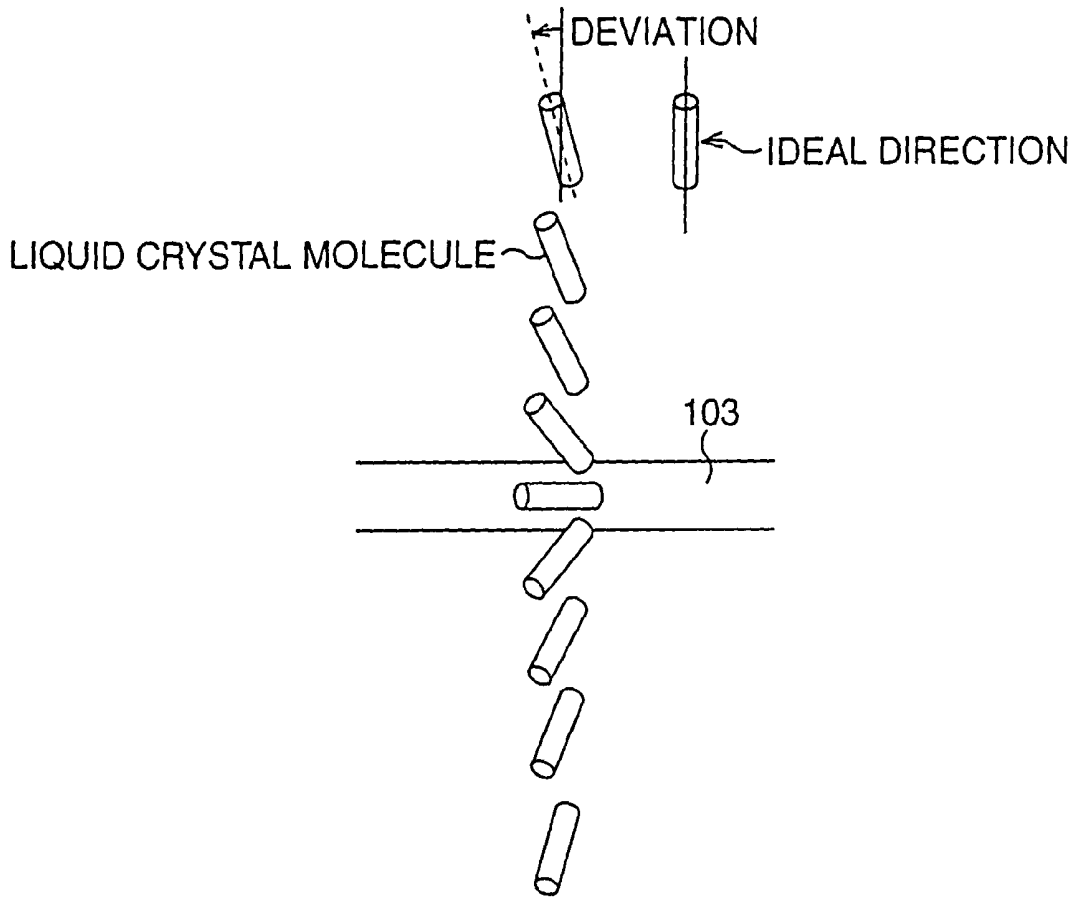
ALIGNMENT DIRECTION OF THE LIQUID CRYSTAL MOLECULE
