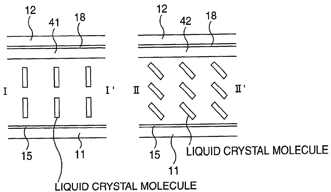
SECTIONAL VIEW
