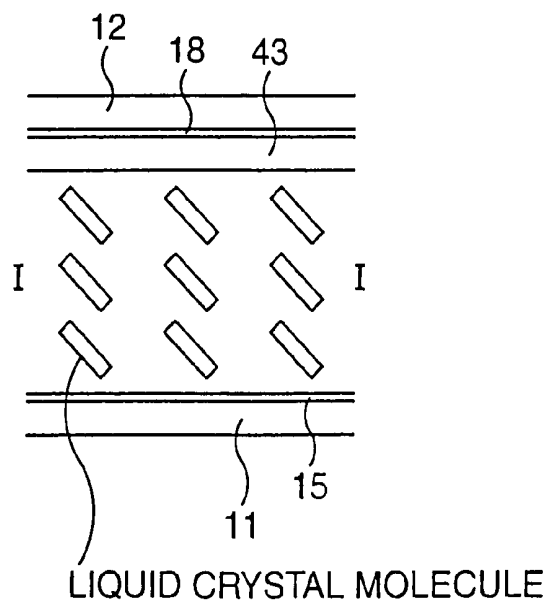
SECTIONAL VIEW
