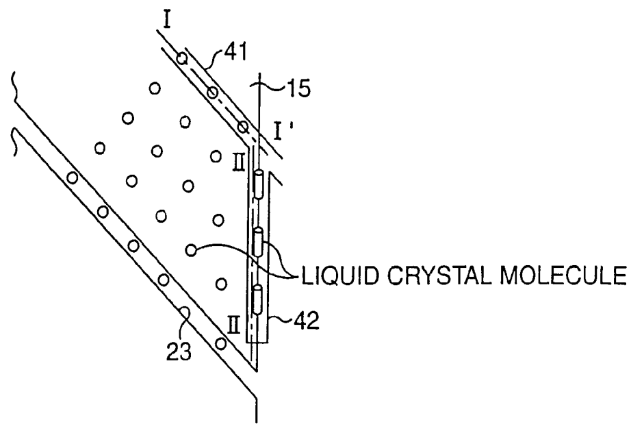
PLANE VIEW
