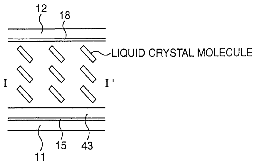
SECTIONAL VIEW
