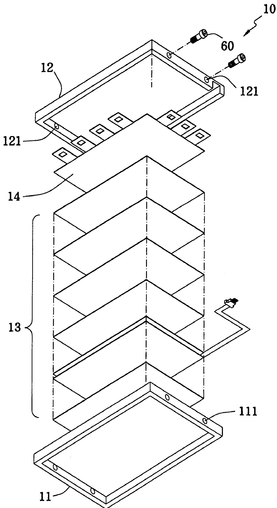
FIG. 1 (Background Art)
