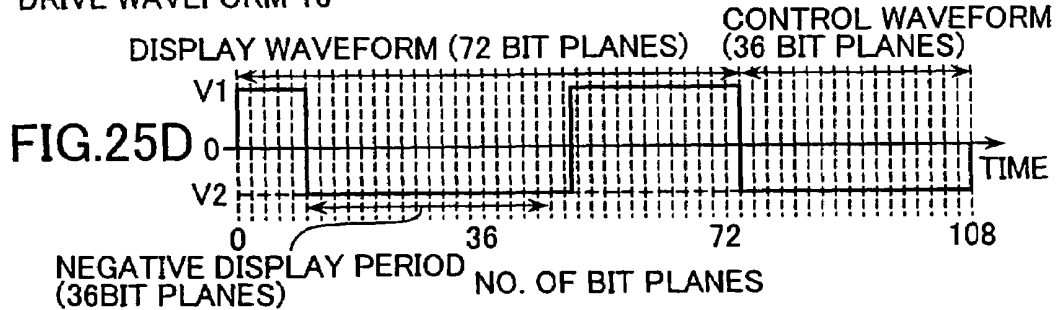
DRIVE WAVEFORM 16
