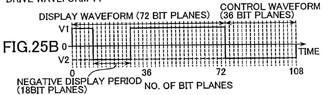
DRIVE WAVEFORM 14
