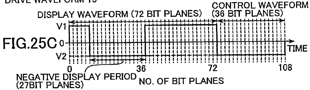
DRIVE WAVEFORM 15
