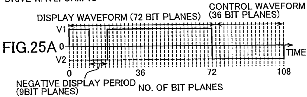
DRIVE WAVEFORM 13
