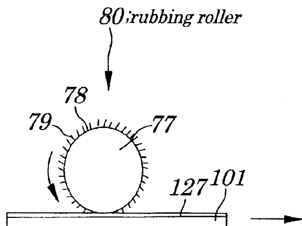
FIG. 12 (PRIOR ART)
