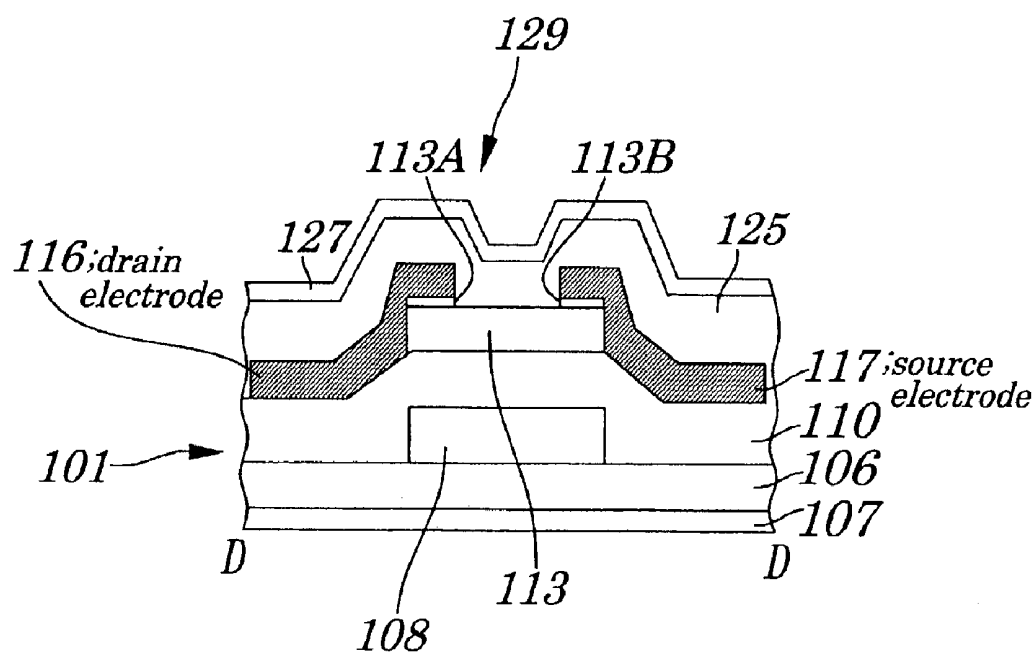
FIG. 11 (PRIOR ART)
