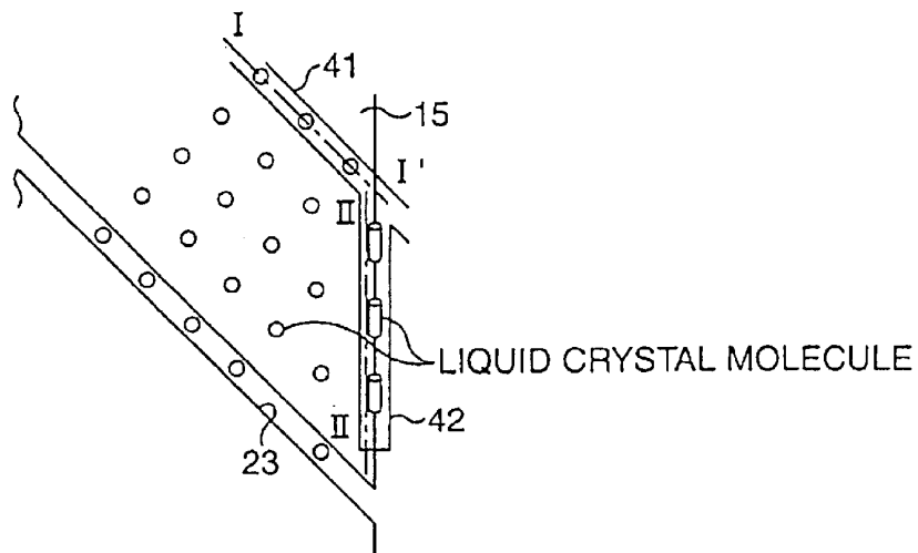
PLANE VIEW
