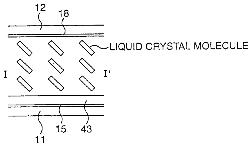
SECTIONAL VIEW
