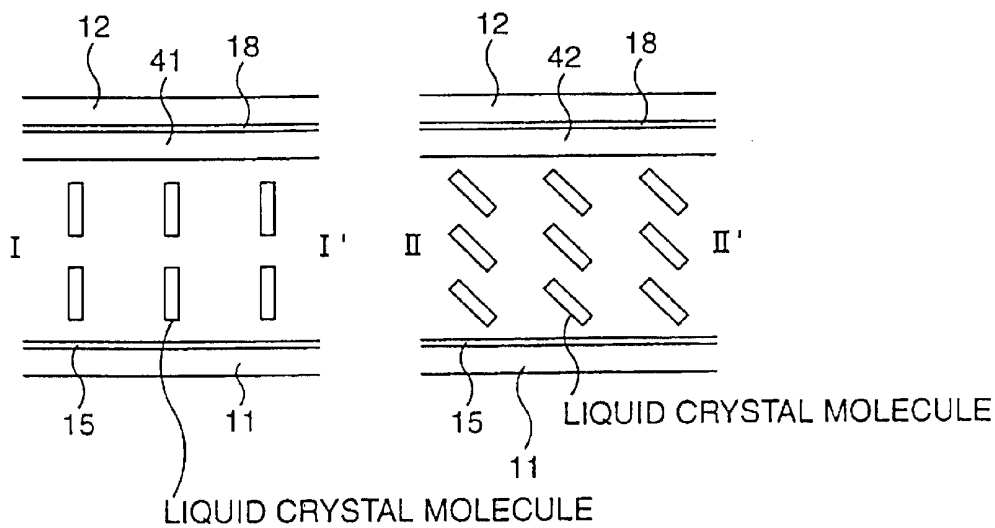
SECTIONAL VIEW
