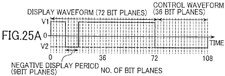
DRIVE WAVEFORM 13
