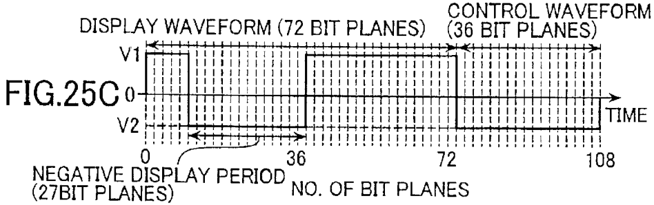
DRIVE WAVEFORM 15
