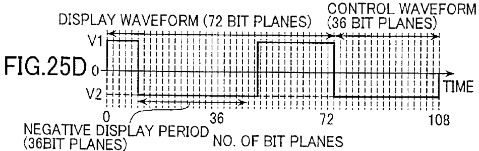
DRIVE WAVEFORM 16
