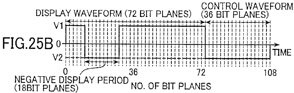
DRIVE WAVEFORM 14
